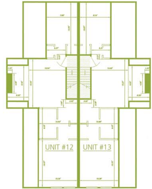
Attic Floor
