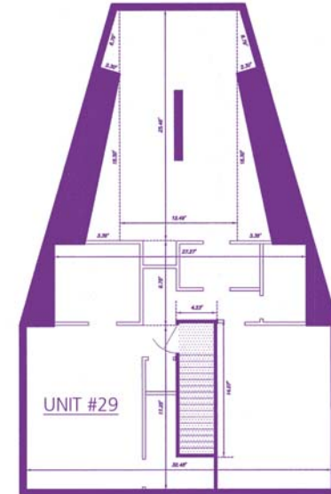
Third Floor
