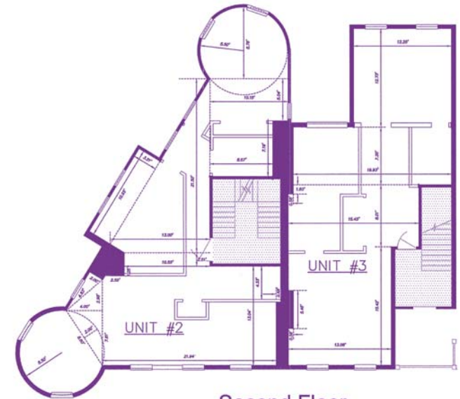
Second Floor
